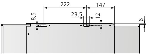
Figure 20. Dimensions de suspension
