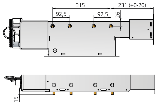
Figure 23. Dimensions de suspension
