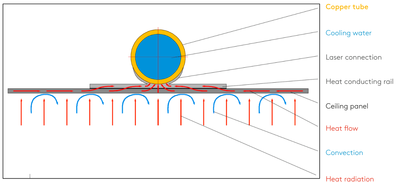
Fig. 1: Basic operating principle of a radiant ceiling
