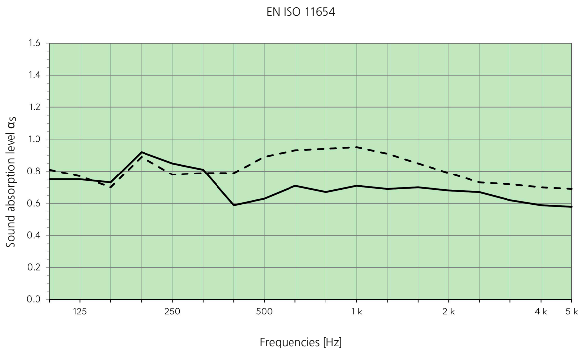
Fig. 6: Sound absorption curve over different frequencies using the example of a metal radiant ceiling with acoustic fleece and mineral wool mat — without acoustic fleece and mineral wool mat -- with acoustic fleece and mineral wool mat
