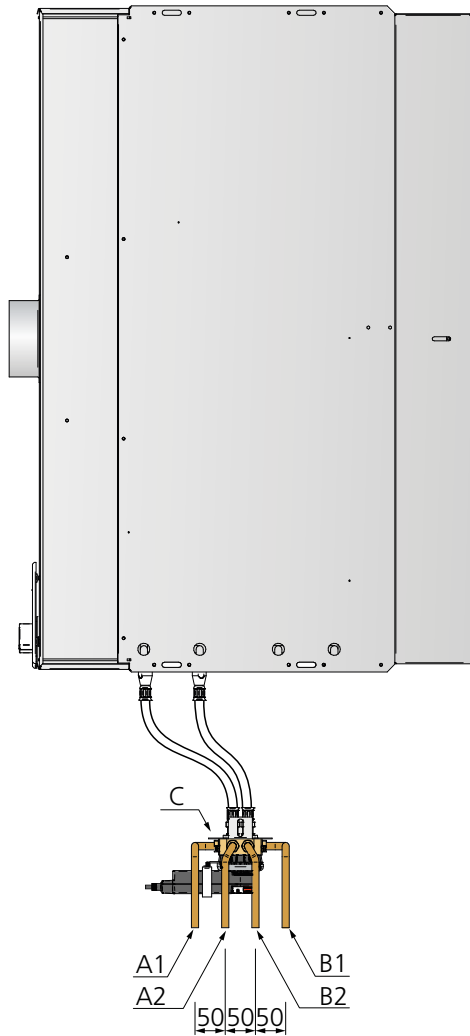
Figure 23. Raccordement hydraulique, vanne CCO.
