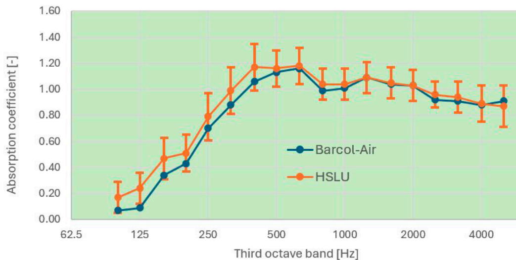
Comparison of Barcol-Air reverberation chamber with HSLU ceiling sail, installation height 200 mm
